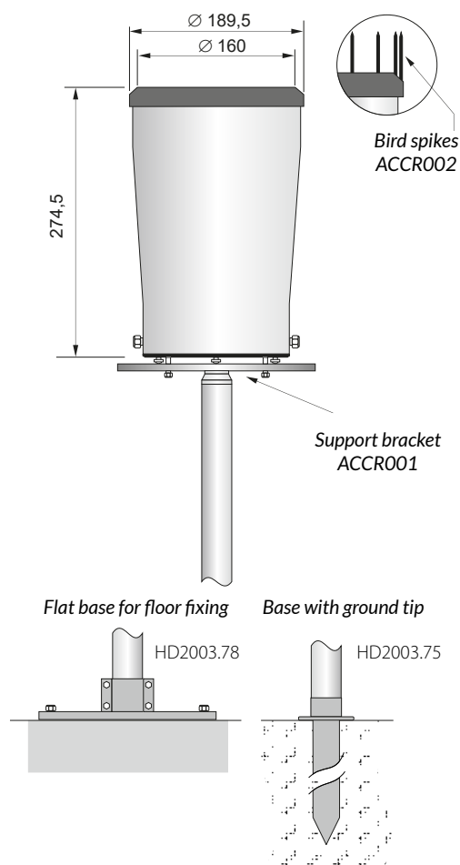
Ground installation
