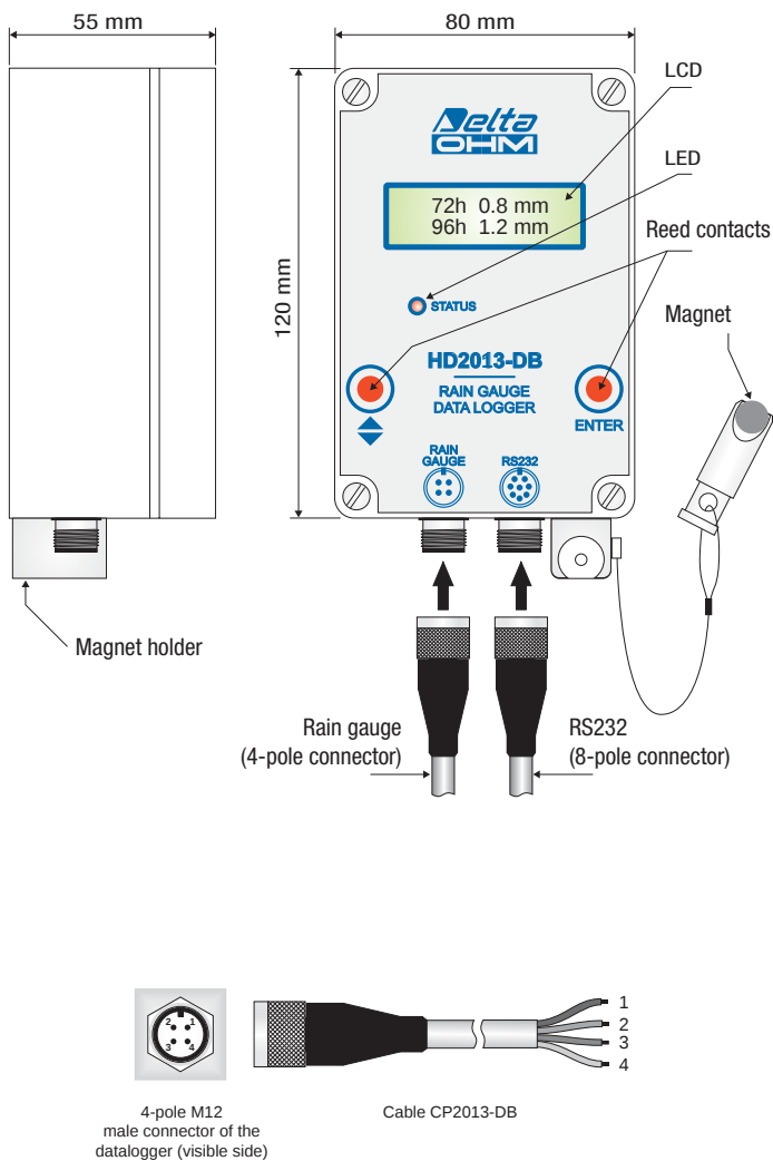
Fig. 2: Description and connections
