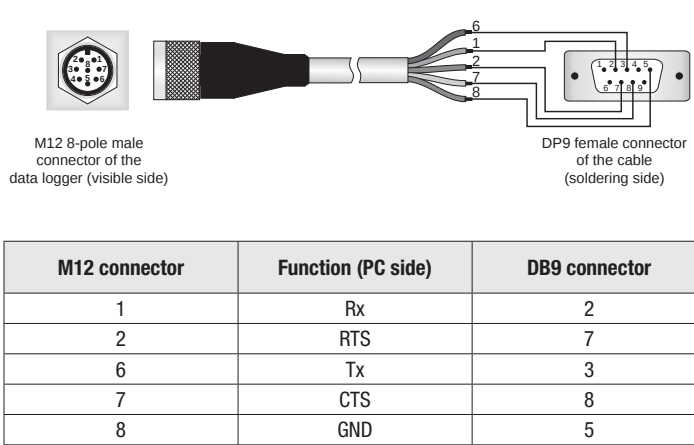
Fig. 4: RS232 Serial connection
